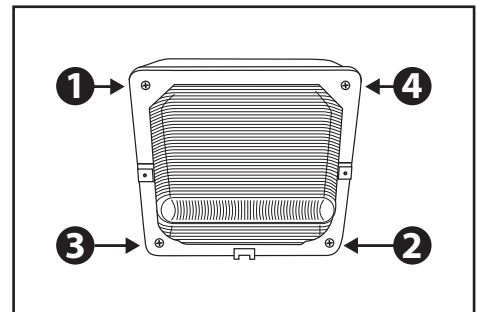
STEP 6: Close front housing by tightening the screws using the following pattern.
