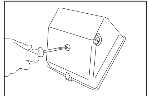
STEP 3: Remove knockout plug on the back of the fixture. Pull supply wires through mounting plate and make connections as noted in the wiring section. Attach to mounting box. Seal with weatherproof silicone sealant to prevent moisture from entering the fixture
